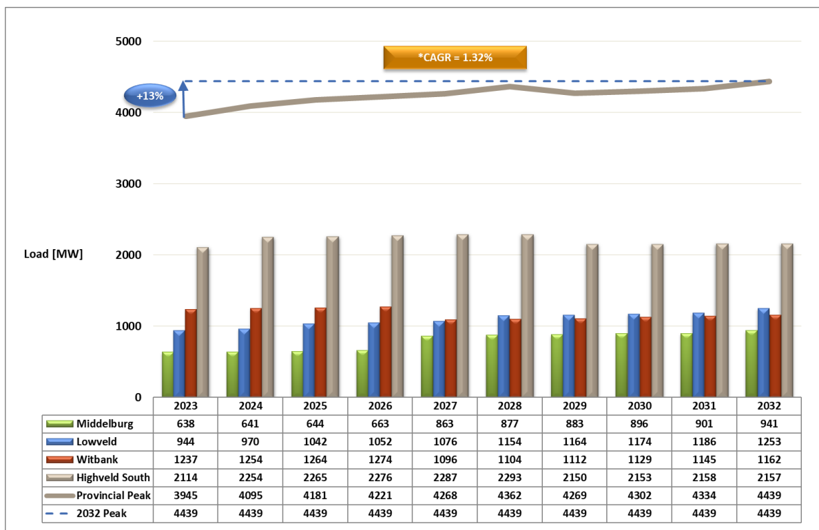
Figure 7-19: Mpumalanga load forecast
