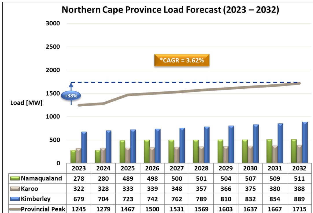
Figure 7-22: Northern Cape load forecast
