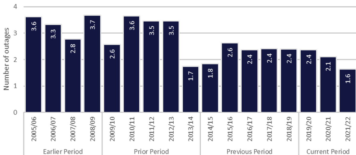
Figure 2.3: SAIFI 2005/06 to 2021/22
