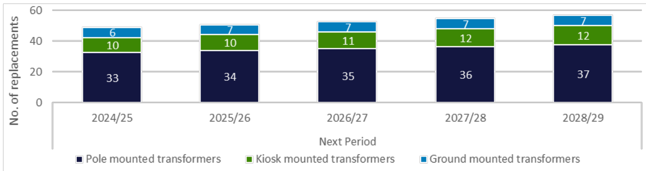
Figure 6.9: Quantities of distribution substation replacements (quantity)
